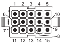
REAR VIEW OF CONNECTOR
