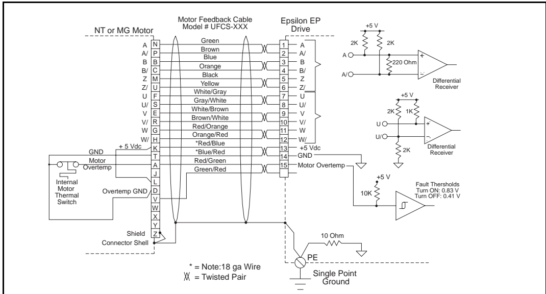
Figure 28: Motor Encoder Feedback Connector Pinout
