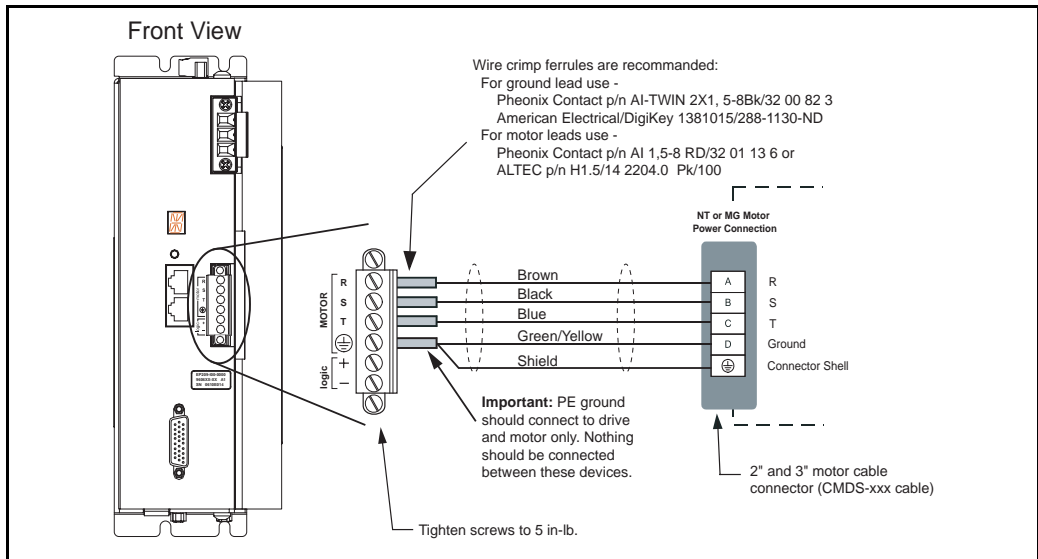
Figure 21: Epsilon EP209 - NT/MG Motor Power Wiring Diagram
