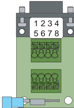
Figure 39: STI-SNCI Interface Board
